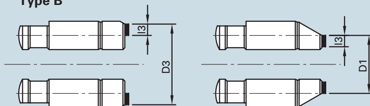
size 35 – 6 with carbide inserts Type B
