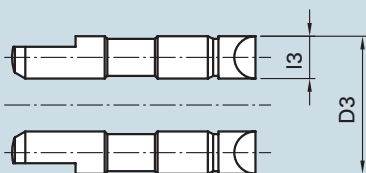
size 01 – 3 made of full carbide Type A
